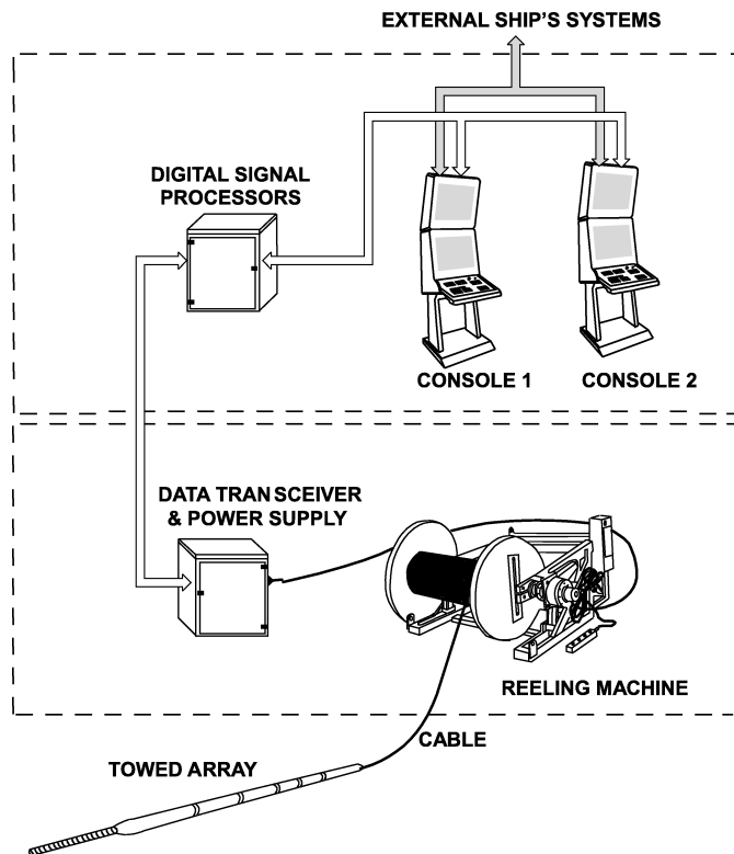
Fig. 2. Sonar structure.
