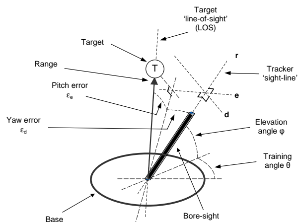
Fig. 1. Tracker angles.
