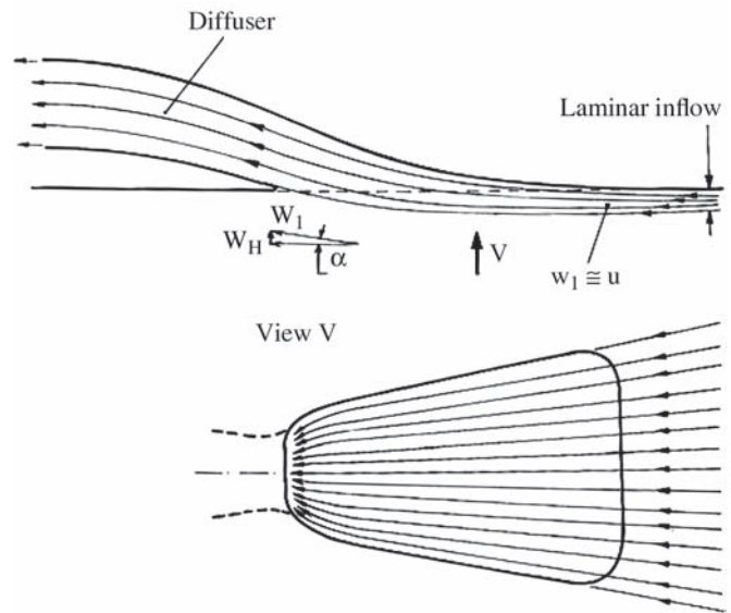
Fig. 1. Laminar water flow into diffuser.
