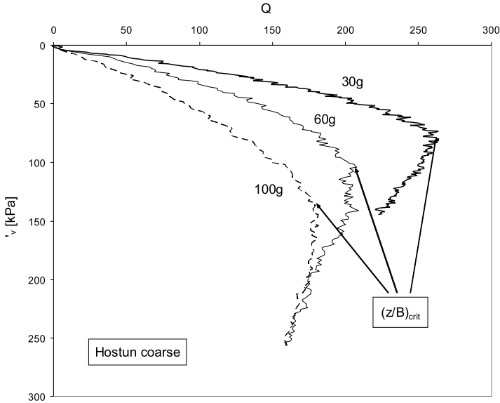
Fig. 18. Normalized cone resistance in coarse sand
