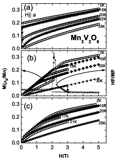
FIG. 3. \text{Mn}_3\text{V}_2\text{O}_8 M(H) isotherms for (a) H \parallel a , (b) H \parallel b , and (c) H \parallel c (left axis) and the H \parallel b T=2\text{K} dM/dH curve [crosses, right axis (b)].
