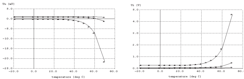
Fig. 3. DC offsets in voltage and current measurement paths for different range resistors: o – R_R = 10 \text{ M}\Omega , x – R_R = 100 \text{ M}\Omega , a – R_R = 1 \text{ G}\Omega .
