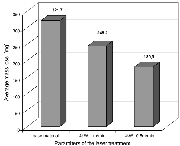
Fig. 8. Average mass loss of the SUPERSTON alloy remelted in the different conditions
