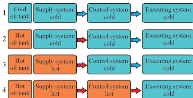
Fig. 1. Four cases of starting conditions of a hydraulic system at low ambient temperature
