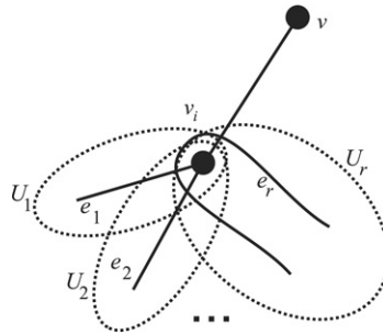
Fig. 3. Hypertree S_p and its subhypertrees U_1, U_2, \dots, U_r .
