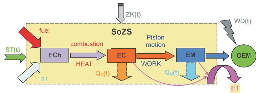
Fig. 1. Example diagram of energy conversion for a diesel engine: ST(t) – engine control, E_{Ch} – chemical energy, E_C – thermal energy, E_M – mechanical energy, ZK(t) – disturbances in engine operation, SoZS – diesel engine, OEM – mechanical energy receiver (e.g. ship propeller, generator, compressor, pump), WD(t) – operating conditions OEM , Q_c(t) – thermal load in time t , Q_m(t) – mechanical load in time t , ET – losses of heat and mechanical energy [8]
