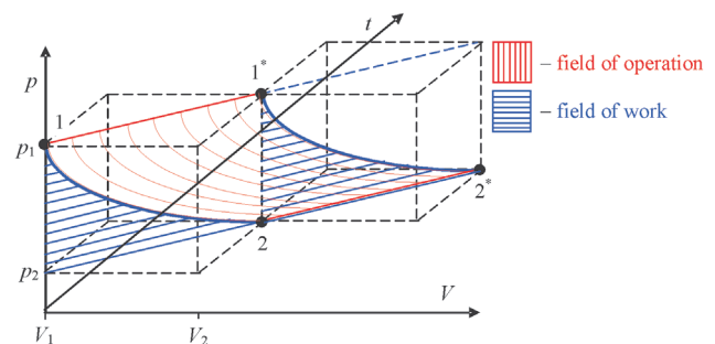
Fig. 4. Graph of technical work and operation of a combustion engine in the “ p-V-t ” system, when the extension time is significant: p – pressure in the workspace, V – volume, t – time, 1 – initial state, 2 – end state, p_1 – initial pressure, p_2 – end pressure, V_1 – initial volume, V_2 – end volume, t_{12} = t_{1+2^*} – time of technical work, t_{11^*} = t_{22^*} – time of engine operation
