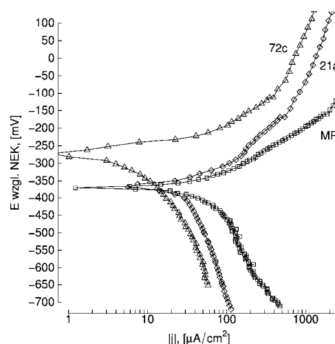
Fig. 3. Potentiostatic curves of the EN AC-AISi12CuNiMg alloy
