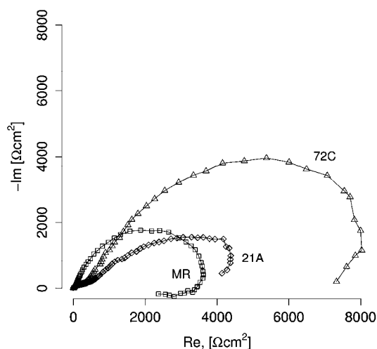
Fig. 2. Impedance curves of the EN AC-AISi12CuNiMg alloy
