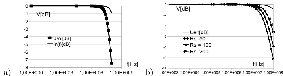
Figure 3. . Influence of measurement circuit properties on achieved frequency band: a) comparison of current and voltage application strategies, b) dependence of frequency band on a quality of the voltage source
