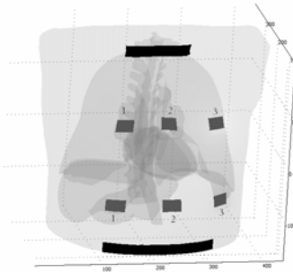
Figure 3. Examined electrode configurations in FEM model.
