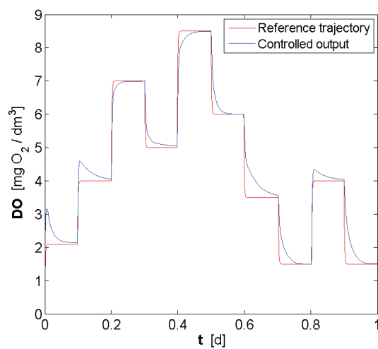
Fig. 13. Closed loop system performance before calibration.
