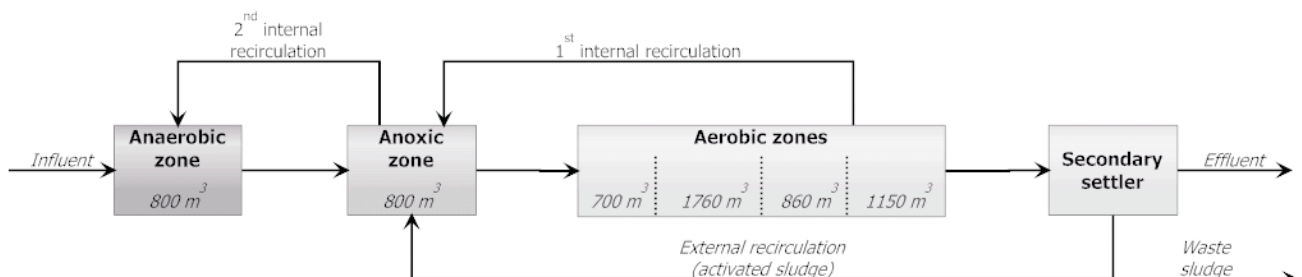
Fig. 1. Scheme of the biological WWTP.
