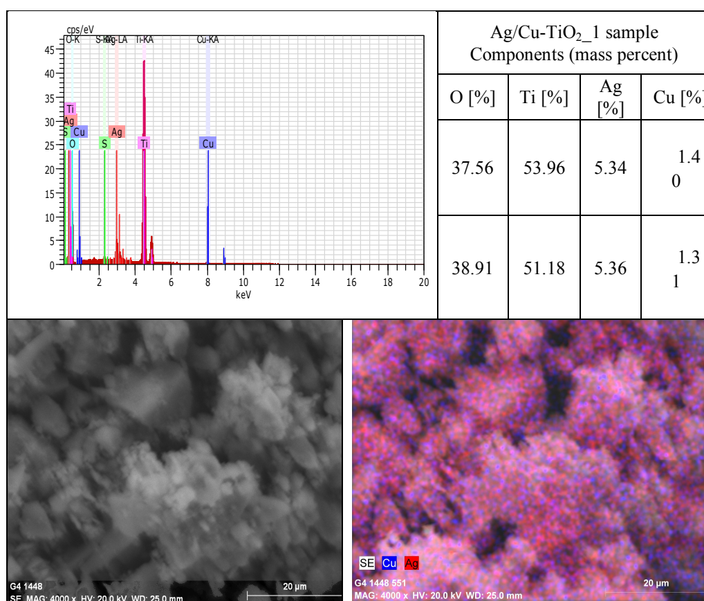
Fig. 4. SEM image and elemental mapping of Ag/Cu- \text{TiO}_2 _4 nanoparticles prepared by microemulsion method
