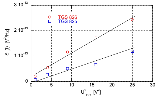
Fig. 3. Power spectral density of voltage fluctuations S_u(f) in gas sensor TGS825 and TGS826 versus squared DC polarization voltage ( U_{DC} ) 2 at a frequency of f=1 kHz and in ambient atmosphere of synthetic air.
