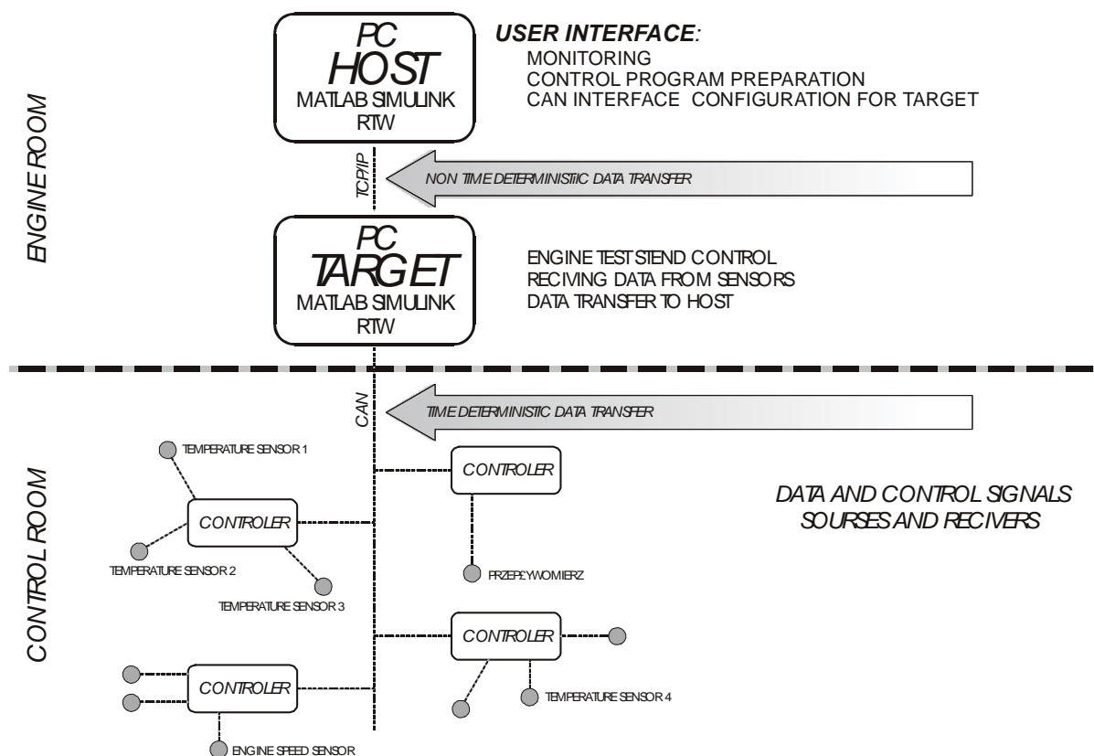
Fig. 1. Diagram of control and data acquisition as a test car engine cooling system
