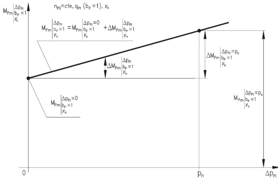
Fig. 2. Torque M_{Pm|\Delta p_{pi}=1, \gamma_n} of mechanical losses in the pump with constant capacity q_{pi} per one shaft revolution ( b_p = 1 ), with working liquid reference viscosity \nu_n as a function of the indicated increase \Delta p_{pi} of pressure in the pump working chambers – graphical interpretation of theoretical model (2)
