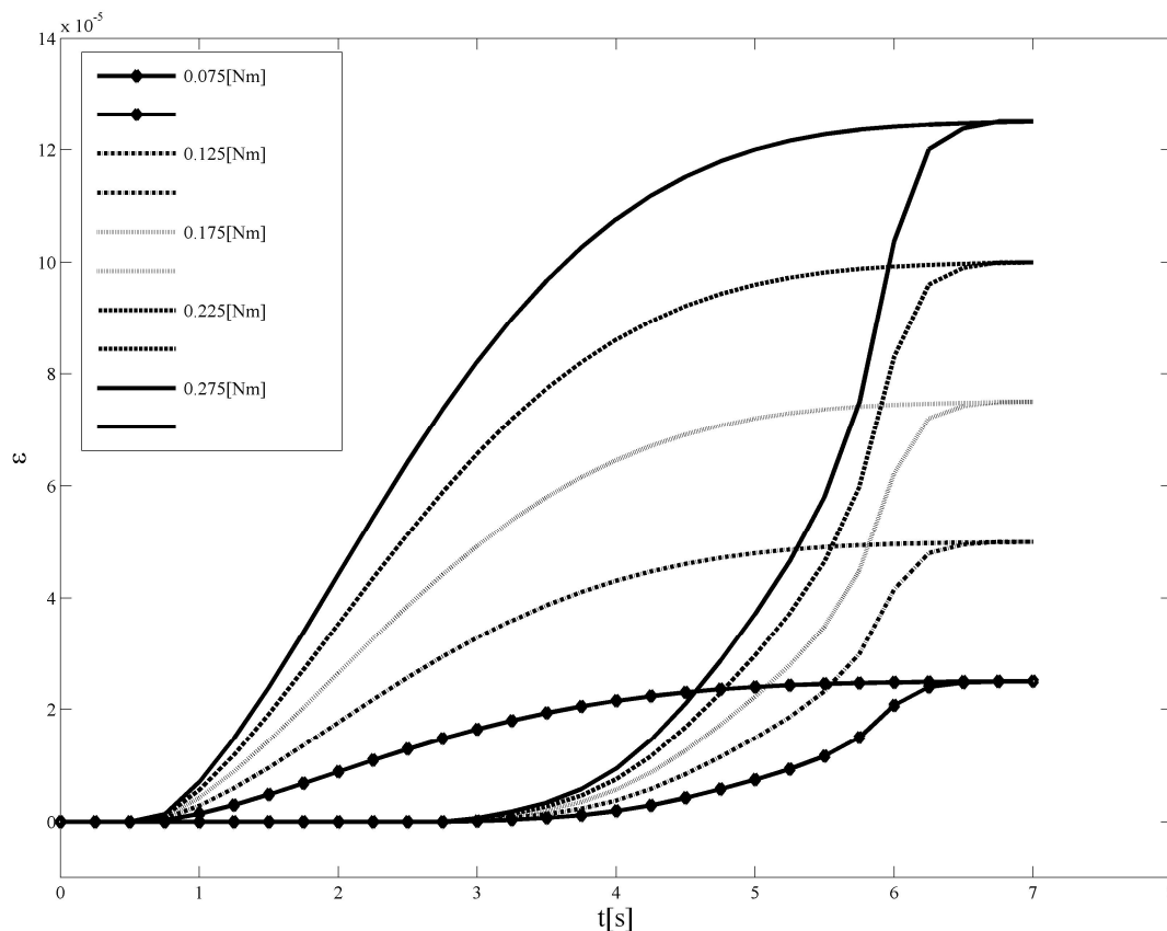
Figure 2. Strain profiles calculated for activation and deactivation processes of one SMA actuator received for different values of the activation moment.
