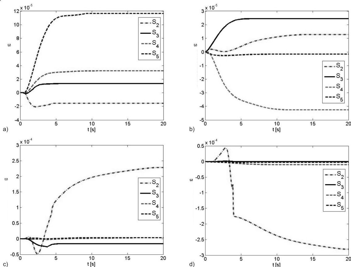
Figure 4. Values of the longitudinal strain measured by FBG sensors ( S_2 - S_5 ) after activation of the SMA actuator (a) A_1 , (b) A_2 , (c) A_3 , and (d) A_4 .
