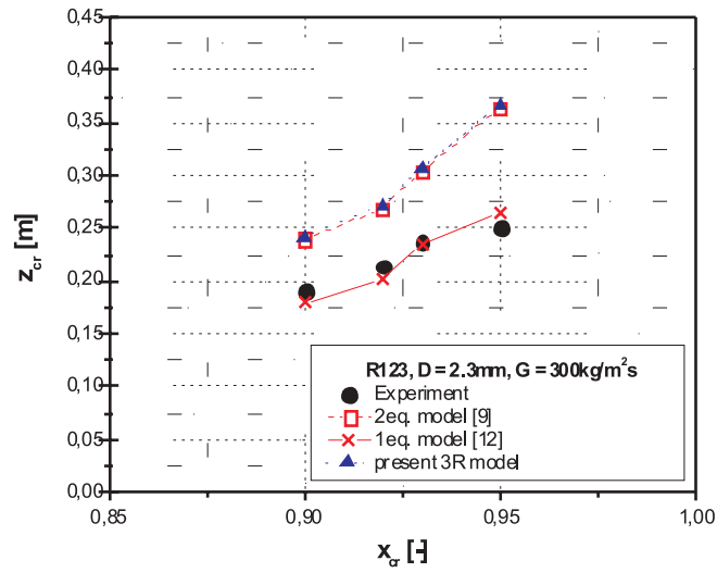
Figure 13. Comparison between the modeling and experimental data for R123 working medium in the channel with D = 2.3 mm and G = 300 kg/m 2 s.
