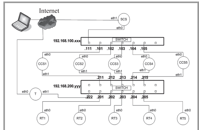
Fig. 6. Architecture and configuration of the implemented ASON/GMPLS testbed.
