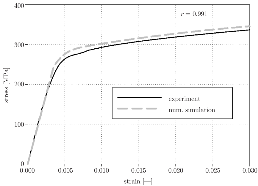
Figure 8. Results of B-P simulation of the uniaxial tension test for \dot{\epsilon} = 5 \cdot 10^{-3} \text{ s}^{-1} , for the specimen cut across the rolling direction of the sheet
