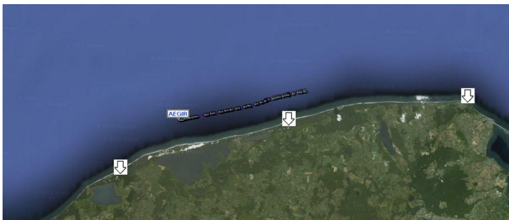
Fig. 7. Visualisation of AEGIR path, ground stations placed along the shore at lighthouses (Czolpino, Stilo and Rozewie)
