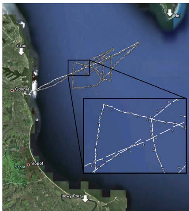
Fig. 4. Deployment of ground stations (arrows) and a path of GPS and GLONASS positions (dotted line) and readings of autonomous AEGIR system (dots)
