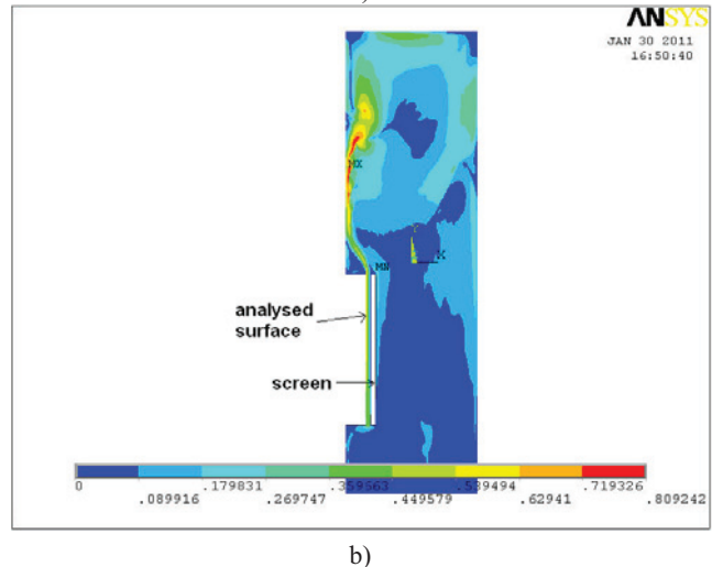
Fig. 3. Air velocity fields – results of simulation investigations of the analysed surface: a) without screen, b) with screen at a distance of x = 4 cm
