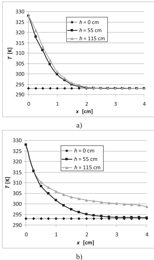
Fig. 4. Air temperature distribution at different heights h as a function of distance x from the analysed device surface: a) arrangement without screen, b) arrangement with screen at a distance of x = 4 cm
