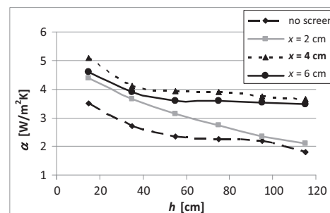
Fig. 7. Distribution of the local heat transfer coefficients \alpha at different heights h for selected distances of screen from the analysed surface: x = 0 (no screen), 2, 4, 6 cm
