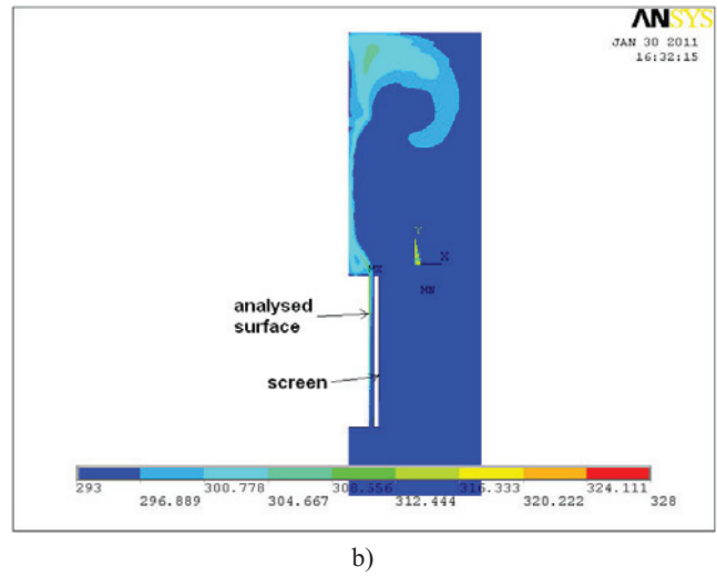
Fig. 2. Air temperature fields – results of simulation investigations of the analysed surface: a) without screen, b) with screen at a distance of x = 4 cm
