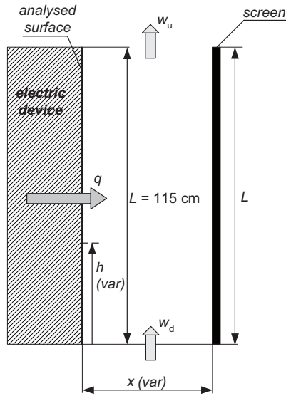
Fig. 1. Diagram of the analysed example; q – heat flux generated by the analysed electric device surface, w_d – air velocity at the system inlet, w_u – air velocity at the system outlet, L – electric device and screen height, h – variable computational height value, x – variable horizontal distance from the analysed electric device surface
