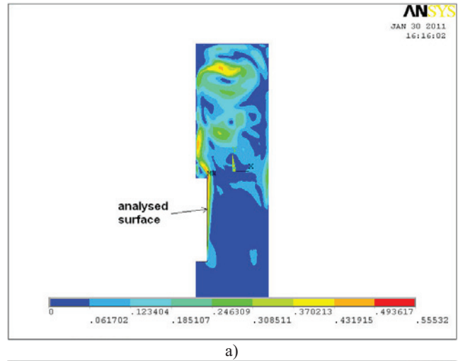
Fig. 2. Air temperature fields – results of simulation investigations of the analysed surface: a) without screen, b) with screen at a distance of x = 4 cm
