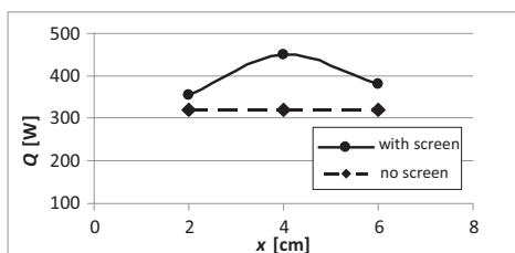
Fig. 8. Transferred energy Q for the arrangement without screen and with screen at a distance of x = 2, 4, 6 , cm
