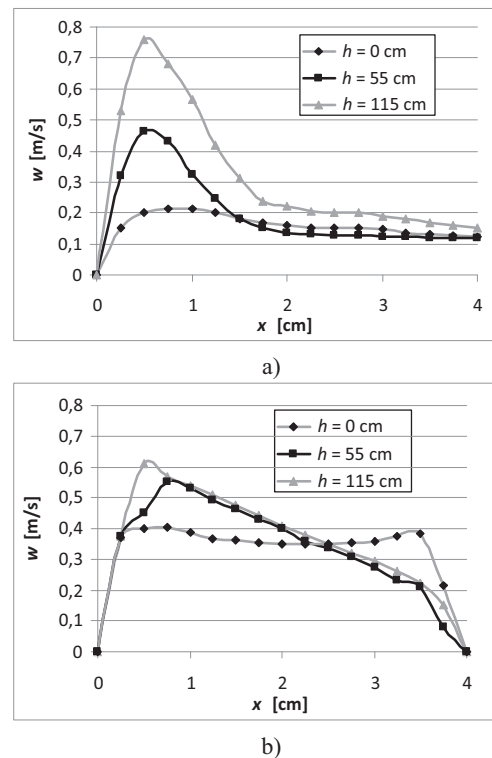
Fig. 5. Air velocity distribution at different heights h as a function of distance x from the analysed device surface: a) without screen, b) with screen at a distance of x = 4 cm
