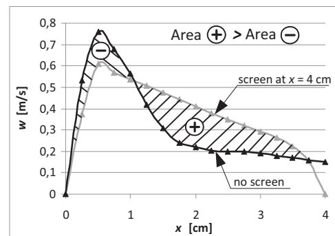
Fig. 6. Air velocity distribution at the height of h = 115 cm as a function of distance x from the analysed device surface, for the arrangements without screen and with screen (screen at a distance of x = 4 cm)
