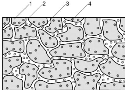
Fig. 3 Greasy lubricant structure diagram: 1 – base oil, 2 – thickener, 3 – additives in the thickener composition, 4 – additives in the oil composition
