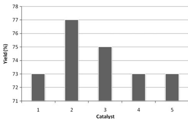
Fig. 4 Phase transfer catalyst influence on yield of theobromine reaction product with 6-chlorohexanone. 1 \text{NEt}_4\text{Br} (73%), 2 \text{But}_4\text{I} (77%), 3 \text{NBzEt}_4\text{Br} (75%), 4 \text{NEt}_4\text{Br} (73%), 5 \text{NMe}_4\text{Br} (73%)
