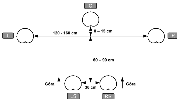
Fig. 2. Microphone placement in the Corey/Martin Tree system.
