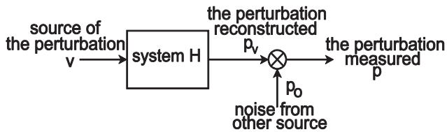
Rys.4. Wiener filtering in estimation of EMI
