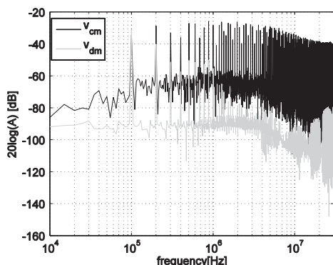
Fig.5. DC-DC boost converter a) generated perturbation spectra b) transfer function (WF approach).
