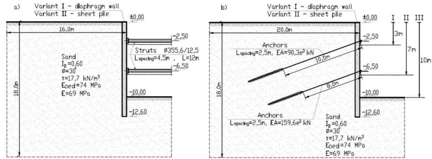
Fig. 5. Geometrical parameters of the deep excavation walls.
