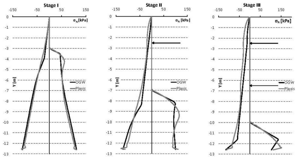
Fig. 8. Soil pressure acting on the diaphragm wall with struts.
