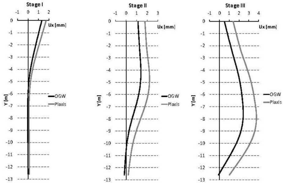
Fig. 7. Horizontal displacements of the diaphragm wall with struts.
