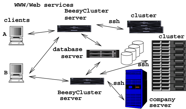
Fig. 6.1: BeesyCluster Architecture
