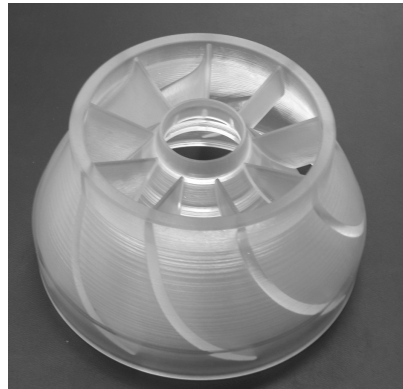
Fig. 2. Exemplary product (pump diffuser) developed with the use of Rapid Prototyping Technology
