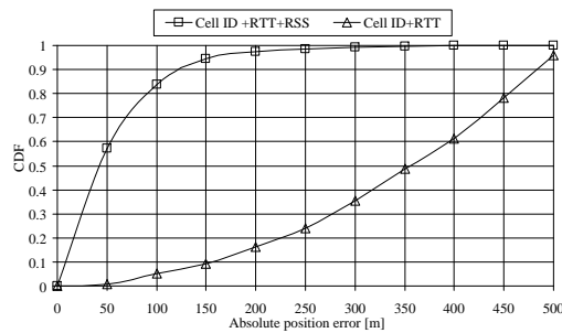
Fig. 5. The CDF of the absolute position error for Cell ID+RTT and Cell ID+RTT+RSS methods.
