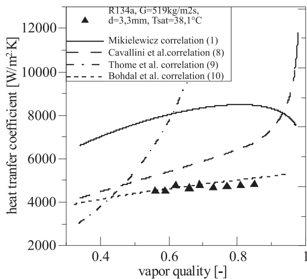
Figure 5. Comparison of heat transfer coefficient for R134a in relation to experimental data due to Bohdal et al. (2011), d = 3.3 mm, G = 519 kg/m 2 s, T_{sat} = 38.1 °C.
