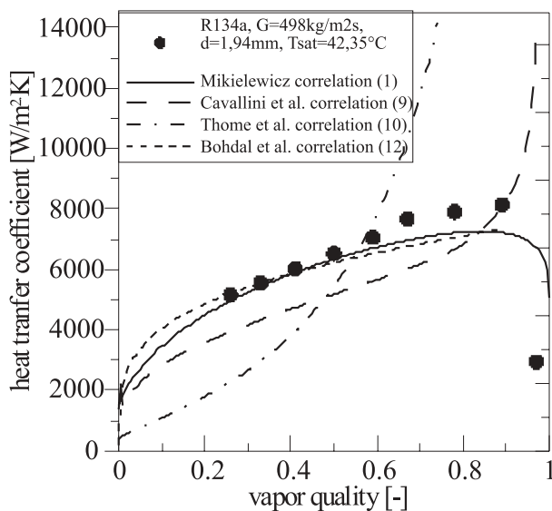
Figure 6. Comparison of heat transfer coefficient for R134a in relation to experimental data due to Bohdal et al. (2011), d = 1.94 mm, G = 498 kg/m 2 s, T_{sat} = 42.4 °C.
