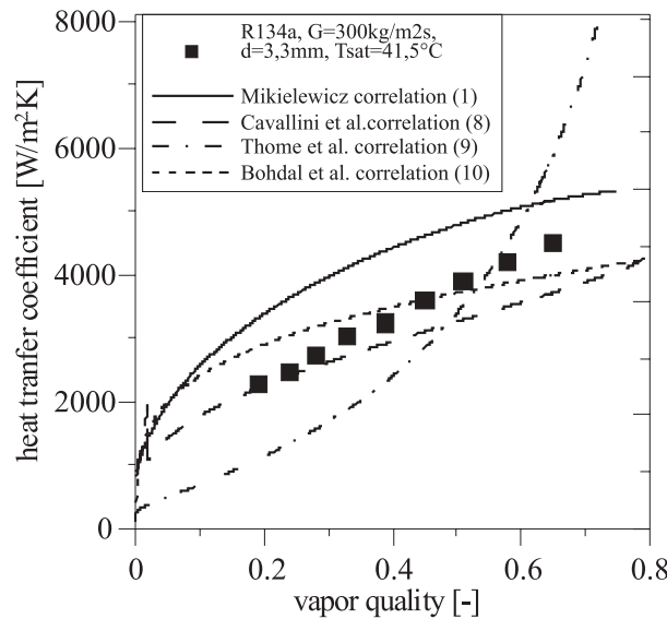
Figure 1. Comparison of heat transfer coefficient for R134a in relation to experimental data due to Bohdal et al. (2011), d = 3.3 mm, G = 300 kg/m 2 s, T_{sat} = 41.5 °C.
