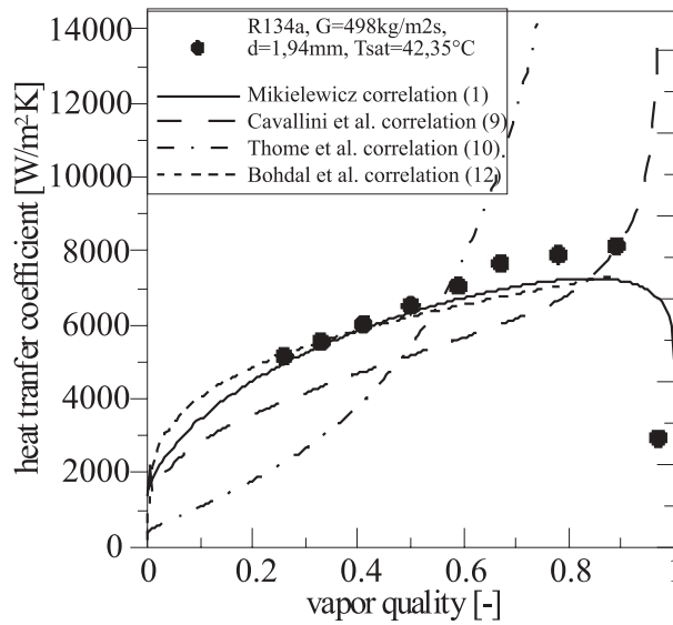
Figure 6. Comparison of heat transfer coefficient for R134a in relation to experimental data due to Bohdal et al. (2011), d = 1.94 mm, G = 498 kg/m 2 s, T_{sat} = 42.4 °C.
