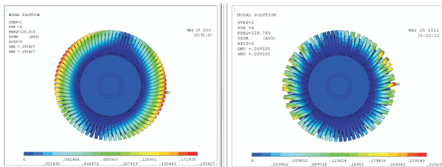
Figure 7 Comparison of mode shapes of the 8th stage bladed disc on shaft corresponding to the one nodal diameter at a frequency of 129 Hz for both cases
