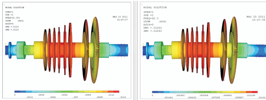
Figure 5 Comparison of mode shapes of tuned and mistuned bladed discs on shaft corresponding to the bending mode of the shaft at a frequency of 62.3 Hz
