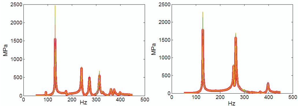
Figure 10 The response of the 8 th stage when the bladed disc is excited by 0EO (left) and 1EO (right) for both cases in the wide range of 50-450 Hz
