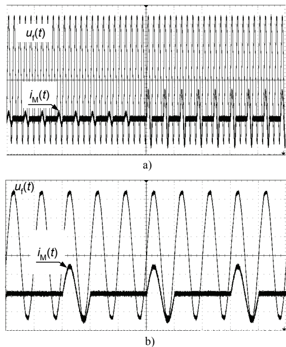
Fig. 6. Oscilloscope of the phase voltage u_f(t) and measurement current i_M(t) of the “Meter-M3”, scale: a) time 100 ms/div, voltage 100 V/div, current 0,5 A/div; b) time 20 ms/div, voltage 100 V/div, current 0,5 A/div
