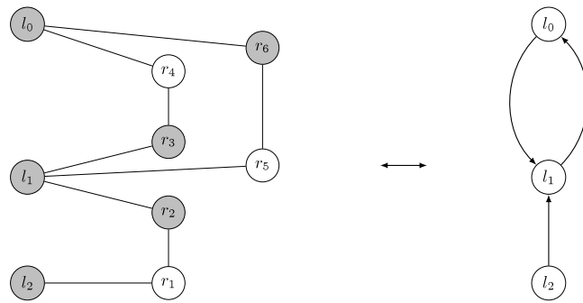
Fig. 2. Correspondence between a special subset of L \cup R and \vec{G}_{L,R} .
