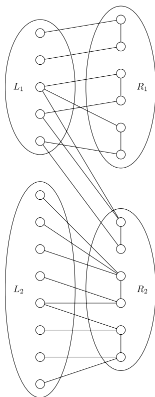
Fig. 5. Illustration of sets L_1, L_2, R_1, and R_2 .
