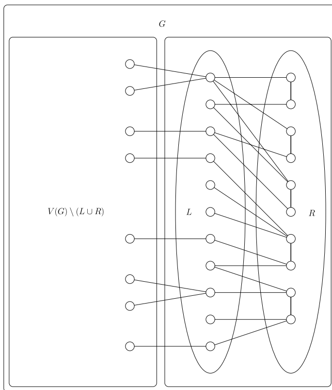
Fig. 7. Partition of V(G) .
