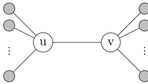
Fig. 6. Vertices u, v with (N(u) \cup N(v)) \setminus \{u, v\} \subseteq S .
