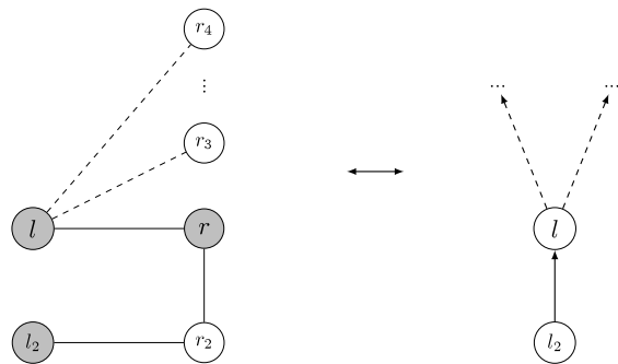
Fig. 3. Vertices l and r are not separated.
