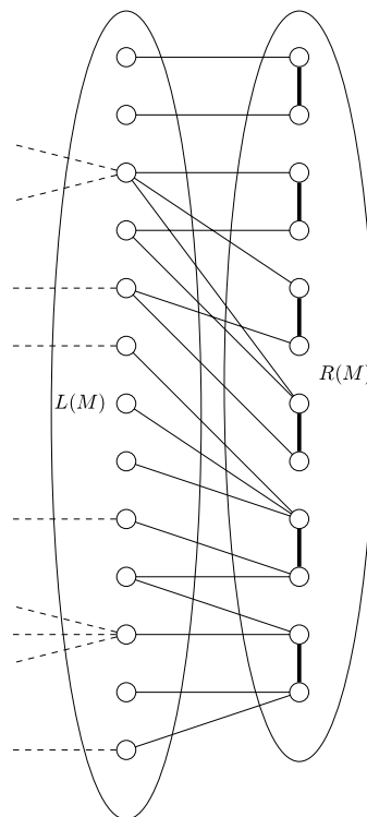
Fig. 1. Example of a strong induced matching M (thick edges) in a triangle-free graph.
