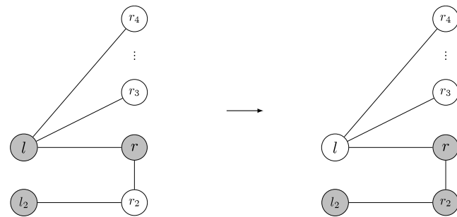
Fig. 4. Local modification of the constructed code.
