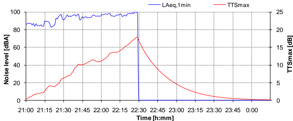
Fig. 11. Equivalent noise levels and maximum instantaneous values of the TTS effect caused by noise observed in typical student club during the 90 minutes exposure.
