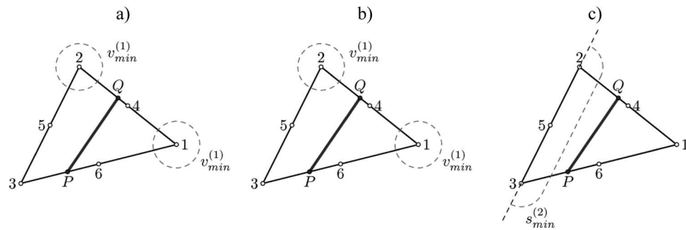
Fig. 2. Minimum distances between crack segments and triangle vertices/sides: a) v_{\min} , b) l_{\min} and c) s_{\min} .
