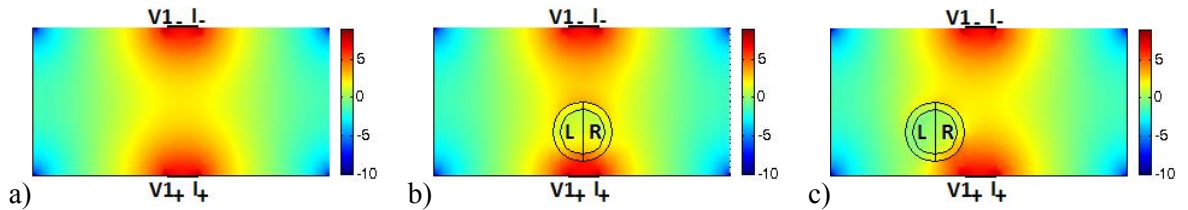
Figure 4. The sensitivity distribution obtained for configuration of electrode-array given in figure 2b.
