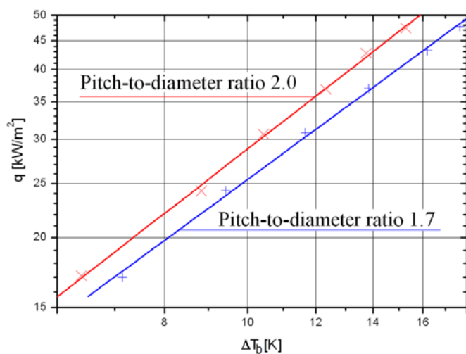
Fig. 6. Influence of pitch-to-diameter ratio for water boiling at atmospheric pressure; pitch-to-diameter ratio: + 1.7, × - 2.0
