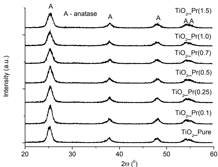
Fig. 3. XRD pattern of \text{Pr-TiO}_2 photocatalysts prepared by sol-gel method
