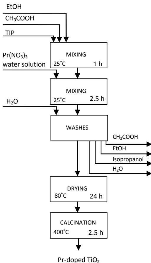
Fig. 1. Block diagram of Pr-doped TiO 2 prepared by the sol-gel method
