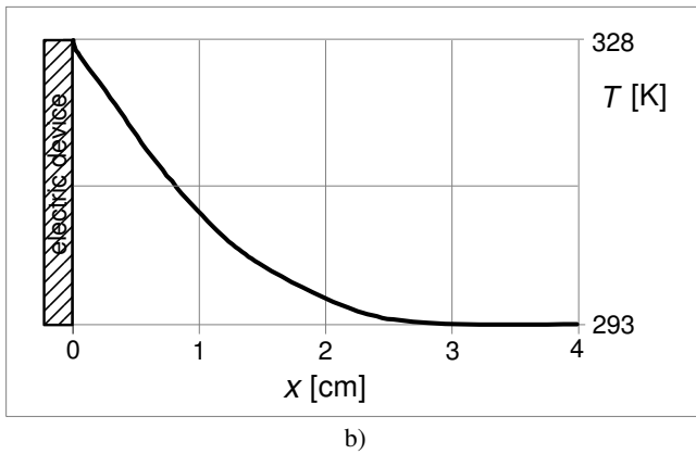
Fig. 7. Air temperature T as a function of distance x from the surface: a) upper left corner c1, b) upper right corner c2; each screen at a distance of x = 4 cm.
