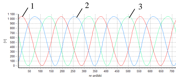
Fig.8. Phase-to-phase voltage of L_1-L_2 , L_2-L_3 , L_3-L_1 as a function of the sample number
