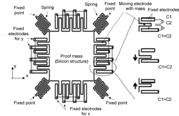
Figure 1. Structure of MEMS acceleration sensor (2-axis) [4].
