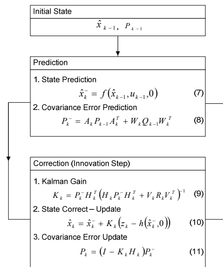
Figure 6. EKF sensor data integration algorithm diagram.
