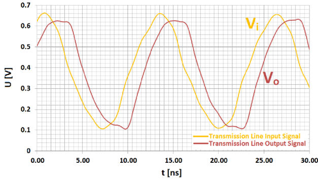
Coupled port
