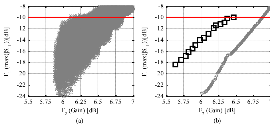
Figure 8: Planar Yagi-Uda antenna: (a) the entire design domain mapped to the feature space; (b) Pareto optimal set obtained for the low- ( \circ ) and the high-fidelity ( \square ) model.
