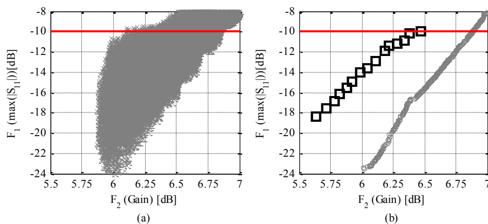
Figure 8: Planar Yagi-Uda antenna: (a) the entire design domain mapped to the feature space; (b) Pareto optimal set obtained for the low- ( \circ ) and the high-fidelity ( \square ) model.
