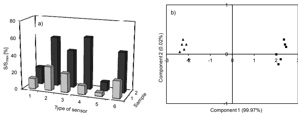
Fig. 8. Mean ratio of the response electronic nose sensors' signal to maximum signal versus sensor type and type of solution: A.1, C.2: a) bar plot, b) linear plot. Type of sensor: 1 – TGS 880, 2 – TGS 825, 3 – TGS 826, 4 – TGS 822, 5 – TGS 2610, 6 – TGS 2602
