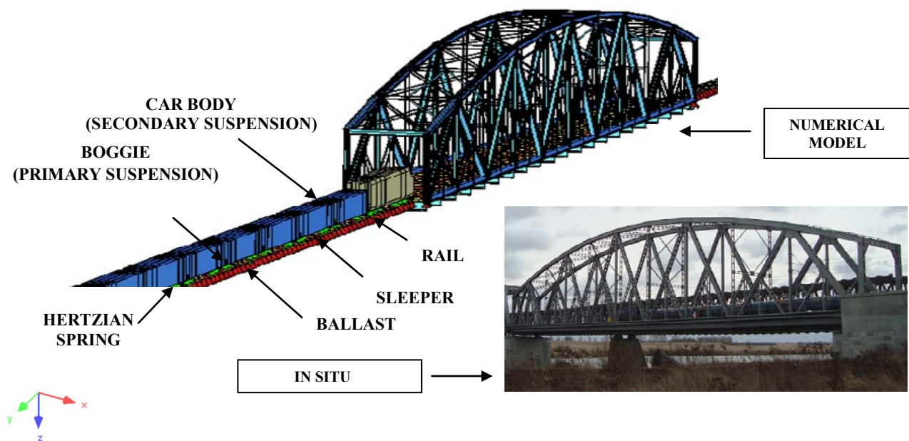
Fig.5. Verification of span model and rolling stock passage.
