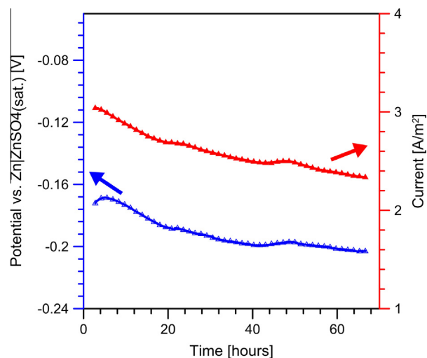
Fig. 3. Cathode potential vs. Zn|ZnSO 4(sat.) and protection current curves for direct anode to cathode connection electrochemical cell.
