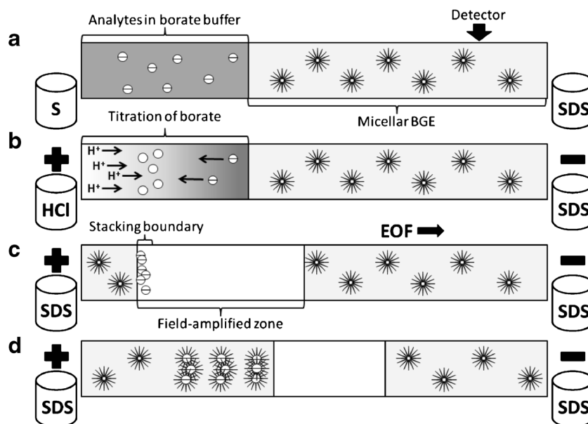
Fig. 2 Pre-concentration of analytes by means of acid-induced pH-mediated technique with hydrodynamic injection of sample. a Initially, the capillary was filled with micellar background electrolyte followed by hydrodynamic injection of a sample. The sample matrix contained borate buffer ( gray area ). b A vial with strong acid solution (0.1 M HCl) was situated at the inlet of the capillary and a high voltage was applied. Electromigration of hydronium ions into the capillary resulted in titration
